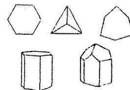
HEXAGONAL
