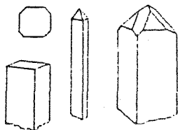
TETRAGONAL
