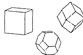
ISOMETRIC
